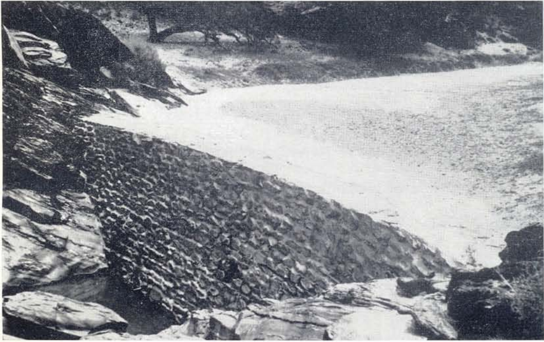
FIG. 1.—An old sand storage dam in the Kuiseb River, South West Africa.
